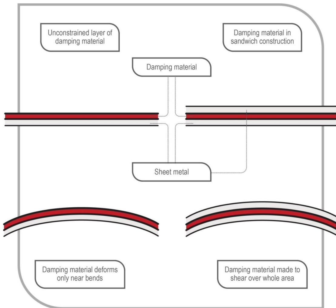
Figure 4 Damping
